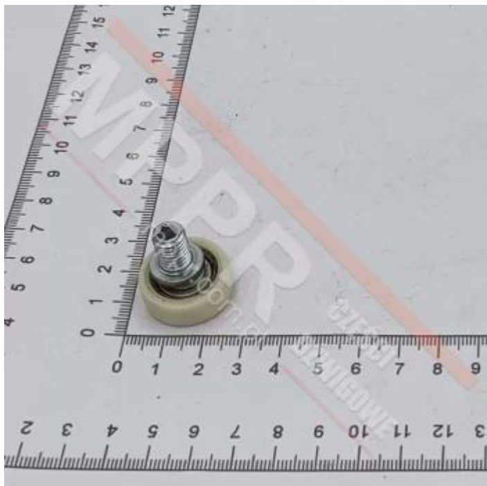
366280 Lower carriage roller for Varidor 20 Door, eccentric M8 x 15 bolt. Ø22 x 8 mm
