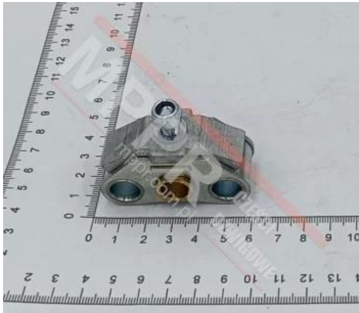
Coupler for belt QKS11 T5/16 CPL
