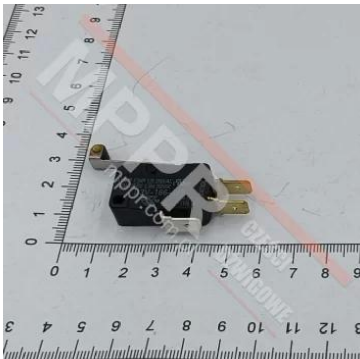
927072 Microswitch for QKS11; 16 A, 250 V, 1CO
