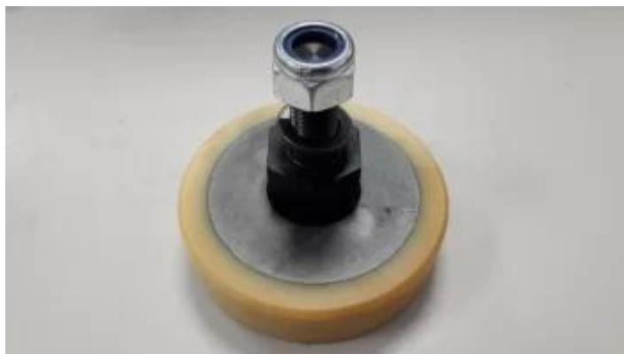
95664300-05 Roller D.125/20X30MM; bearings 6204-2RS + ecentric bolt ACLA THYSSEN
