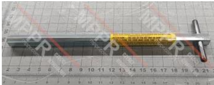
Wittur emergency opening key L = 200 mm
