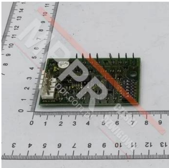
GFA23550D10 Remote station RS-5
