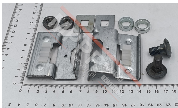
AGH-CVB000000 Set of two guide shoes for car and landing doors
